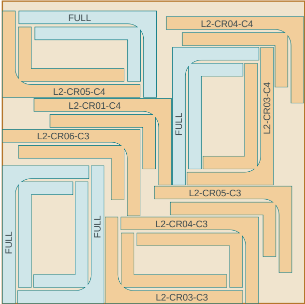
LAYER 3 - L2 courses 3-4 12 forms
