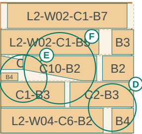
LAYER 8 - L2 courses 1, 2, 4, 6, 9, 10
