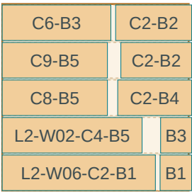
LAYER 6 - L2 courses 2, 3, 5, 10
