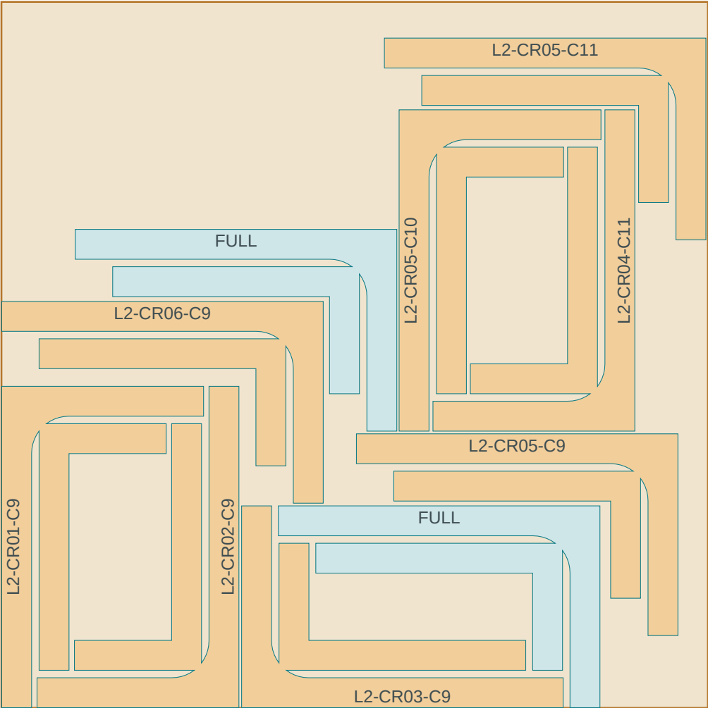
LAYER 1 - L2 courses 9-11
