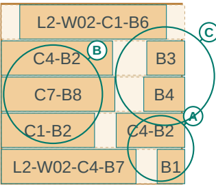
LAYER 9 - L2 courses 1, 4, 7
