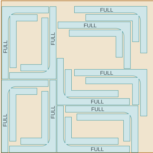
LAYER 3 - L1 courses 2-4 10 forms
