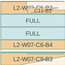
LAYER 3 - L2 courses 6, 8, 9, 11
