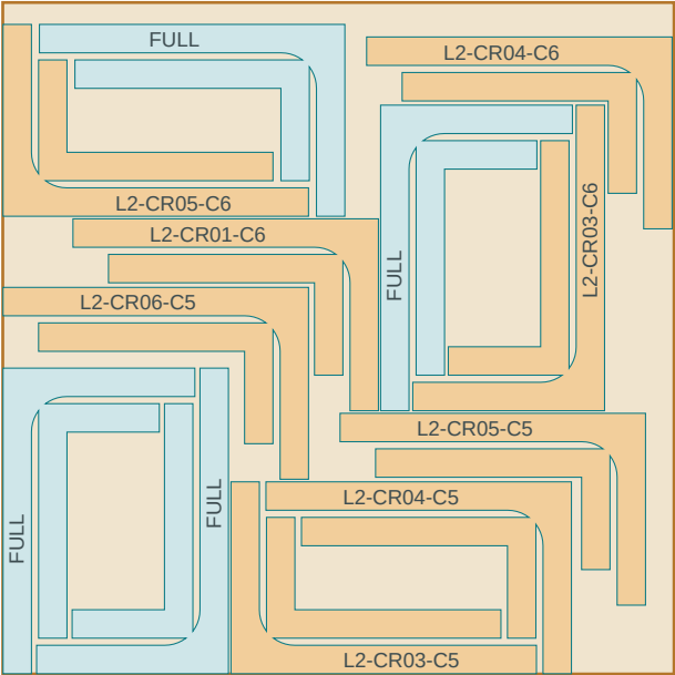
LAYER 2 - L2 courses 5-6 12 forms
